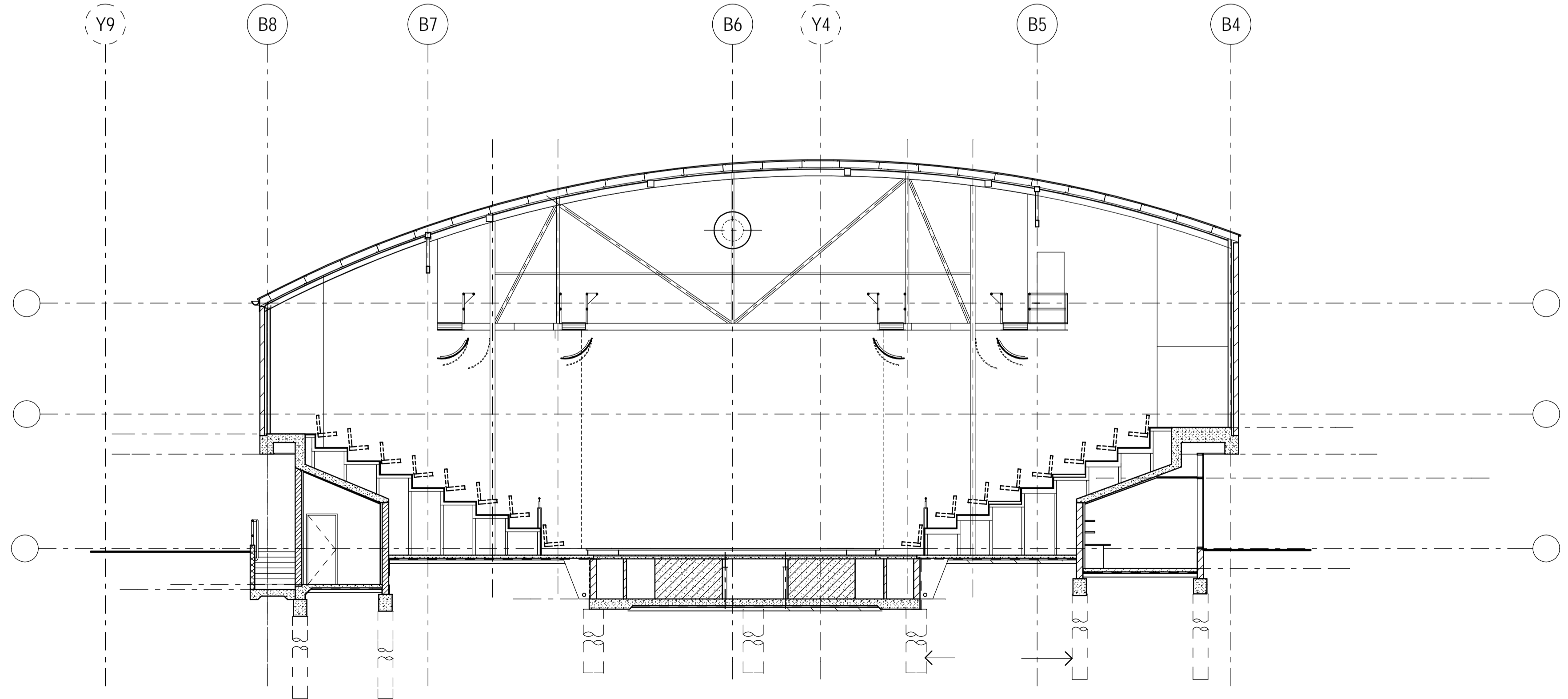
B SECTION : Q THEATRE (STAGE ELEVATION)
