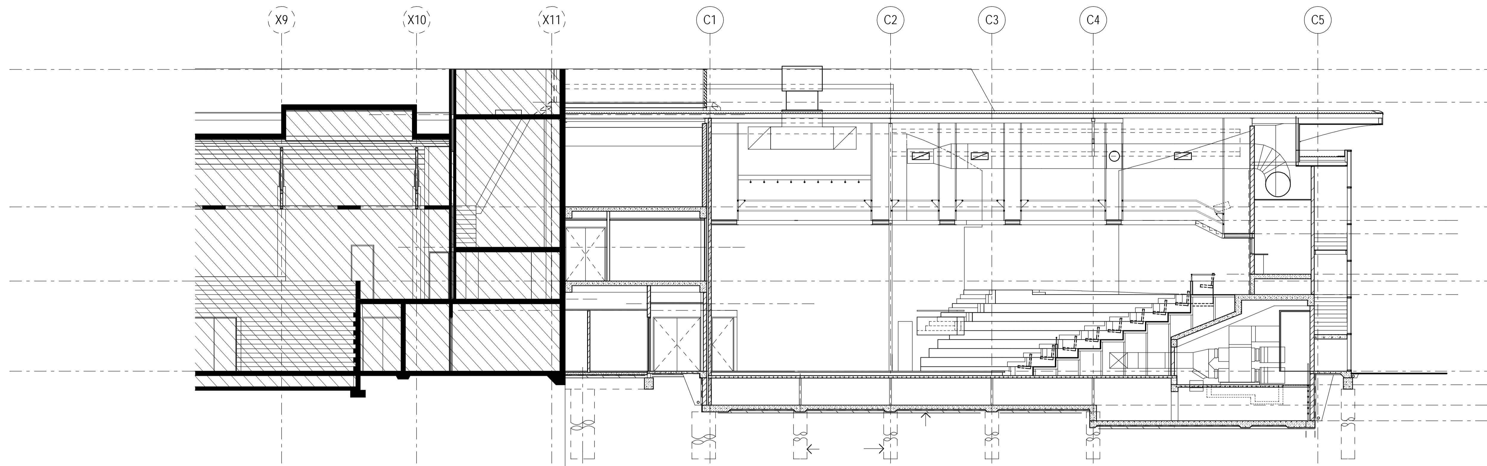
A SECTION : Q THEATRE
